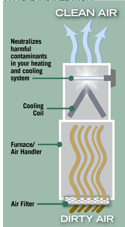
UV1000/2000 TYPICAL INSTALLATION
